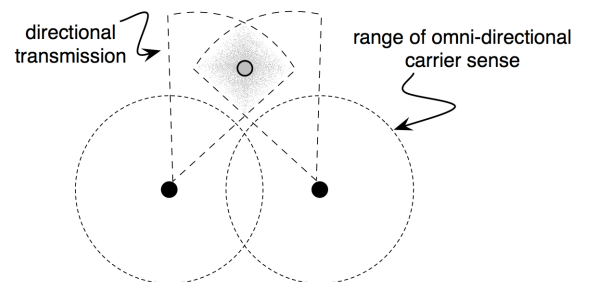
Figure 8: Two nearby transmitters address the same receiver in a directional manner; due to omni-directional CSMA, carrier sense fails and packets collide at the receiver.
