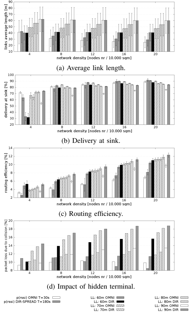
Figure 6: Impact of long links.
