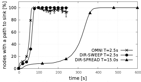
Figure 3: Link probing: convergence time vs. overhead.
