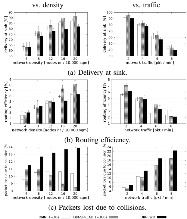
Figure 5: Directional forwarding.
