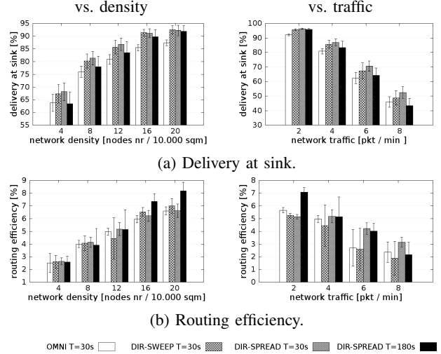
Figure 4: Impact of link probing.
