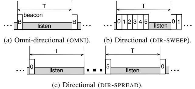
Figure 1: Link probing: node schedule.
