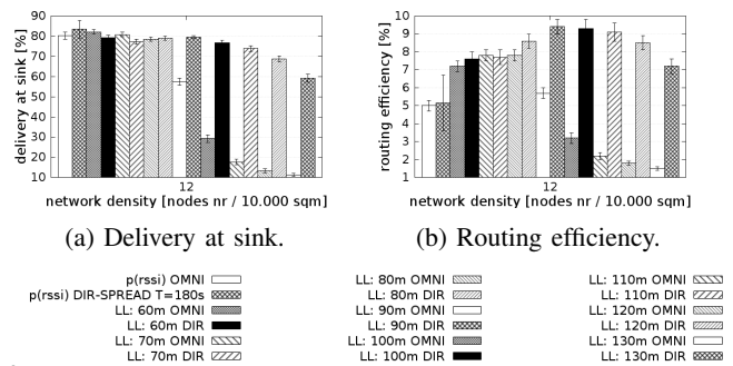
Figure 7: Performance with links up to 130 m, density=12.
