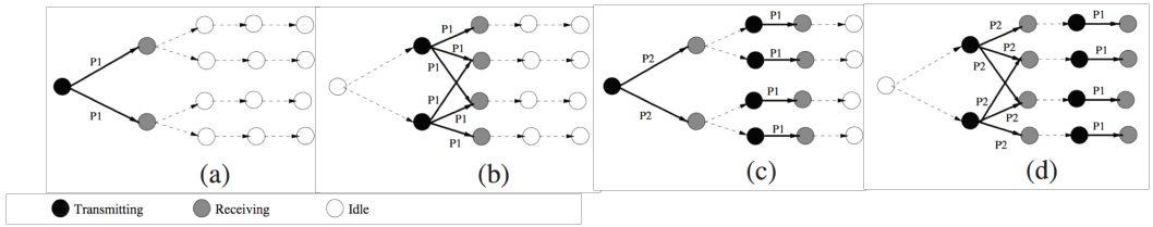
Fig. 5. Splash operation (taken from [27]). Splash creates parallel pipelines, as indicated by packets P1 and P2 in the figure, over multiple paths covering all the nodes in the network. As basis for these parallel pipelines, Splash exploits the routing tree structure previously established by an existing one-to-all data collection protocol.
