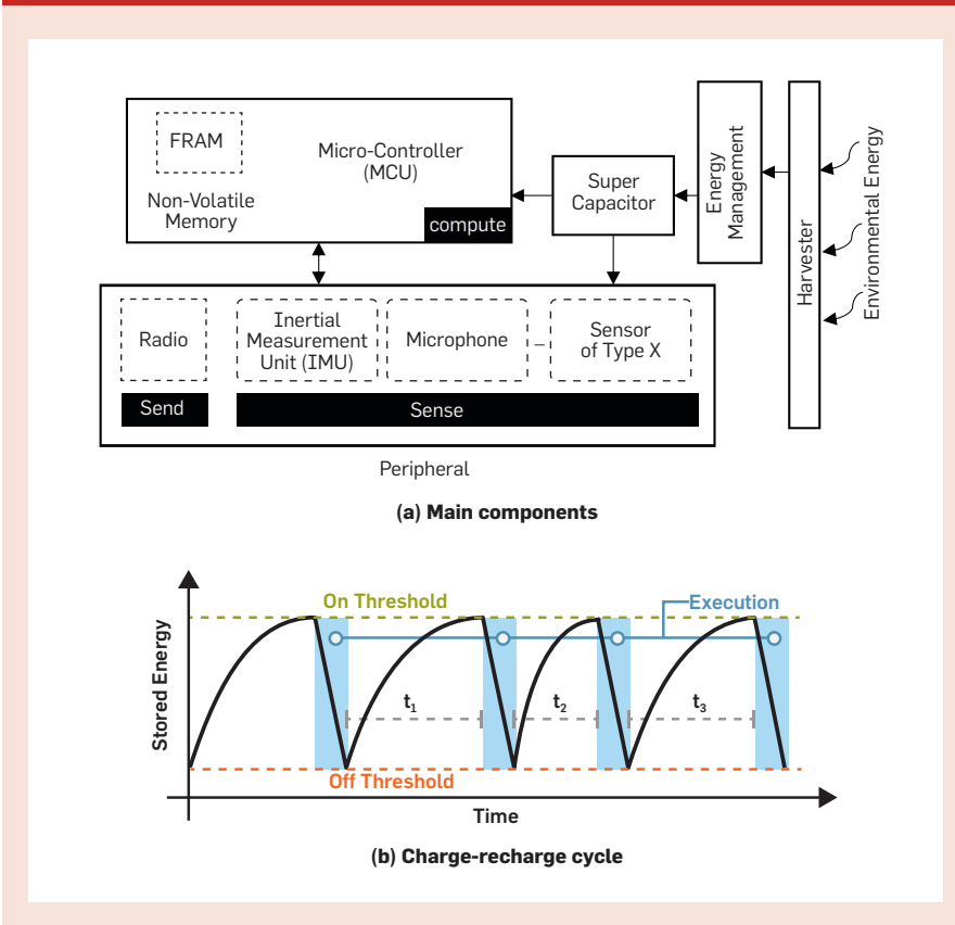
Figure 1. (a) Key components, and (b) Charge-recharge cycle.
