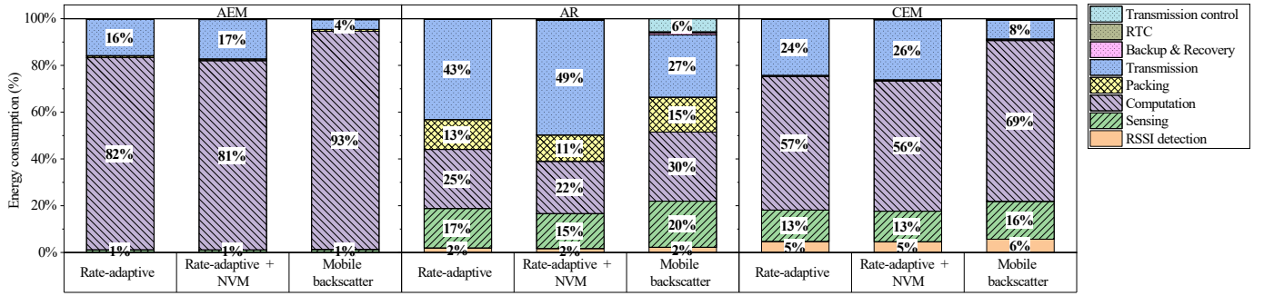
Fig. 7: Energy breakdown per application under the CI_2_C signal trace and jogging node 0 power trace.
