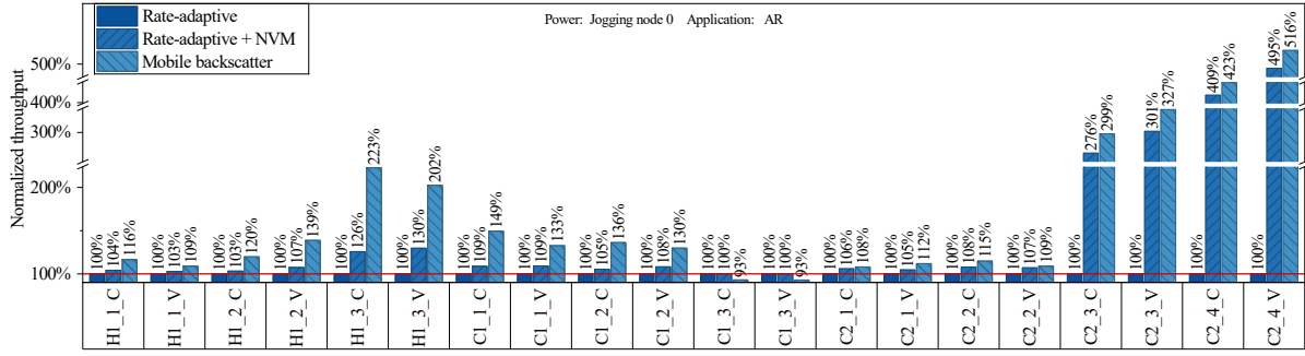
Fig. 3: Normalized throughput per signal trace for the AR application under the jogging node 0 power trace.
