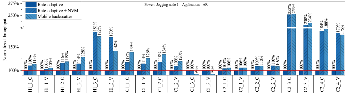
Fig. 5: Normalized throughput per signal trace for the AR application under the jogging node 1 power trace.
