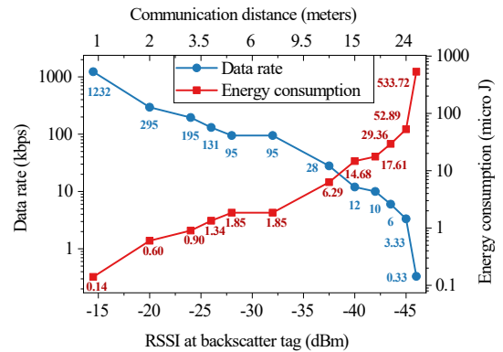
Fig. 1: Impact of channel quality and communication distance on transmission rate and energy cost [13].
