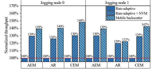
Fig. 4: Normalized average throughput. The mobile backscatter system achieves up to 1.48\times average throughput.
