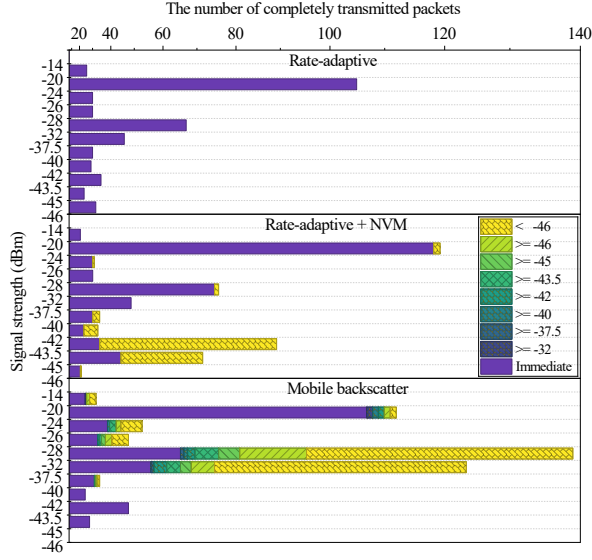
Fig. 6: Comparison of packet transmission behavior across RSSIs for the AEM application under the CI_2_C signal trace and jogging node 0 power trace.
